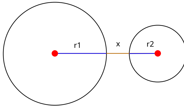
Figure 149: Reference image for Circle-Circle collision detection
